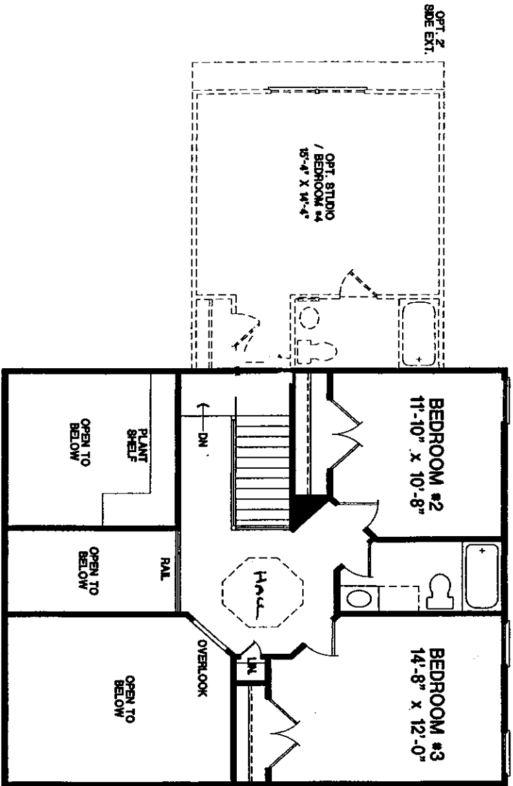
SECOND FLOOR W/ OPTIONAL STUDIO BEDROOM
